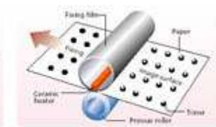
On-Demand Fixing Method
